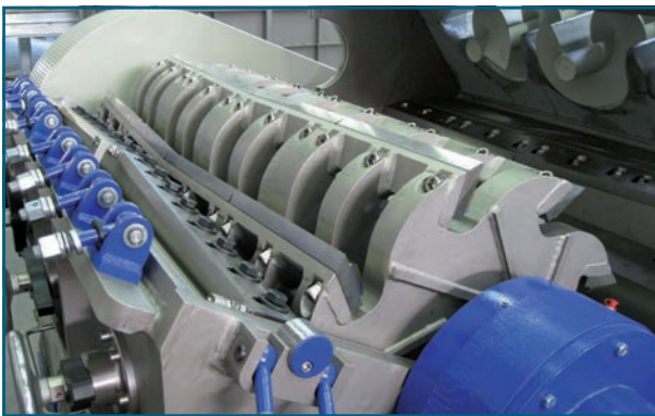
Fig. 1: SMS SB Granulator with Force Feeding Technology
