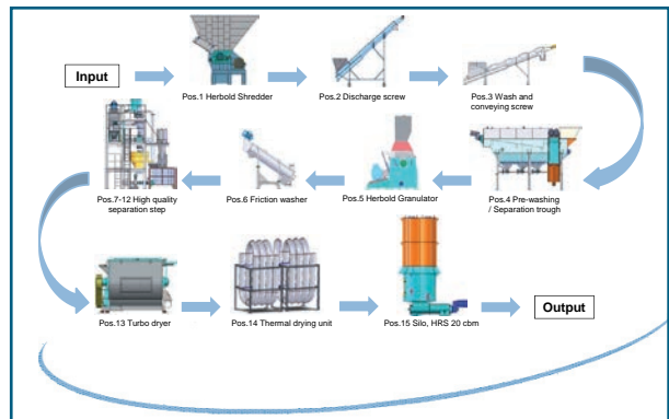
Fig. 4: Flow sheet of a washing line for agricultural film
