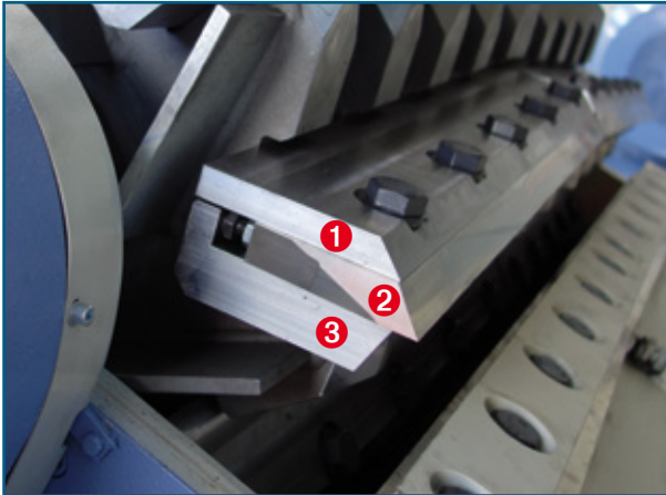
Fig. 3: ① Support plates for knives ② Rotor knives ③ Replaceable wear part
