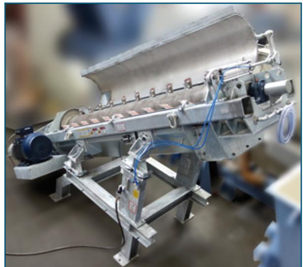
Fig. 9: Pneumatic opening device for maintenance work reduces downtime.
