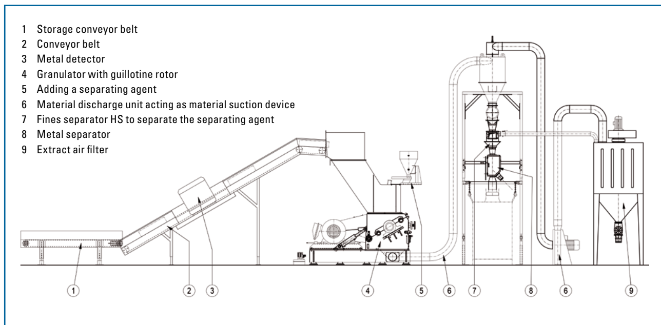
Single-stage size reduction with talcum feed and talcum recovery.
