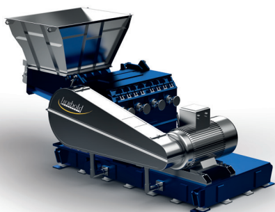
Fig. 1: SMS Granulator of the SB series with forced feeding
