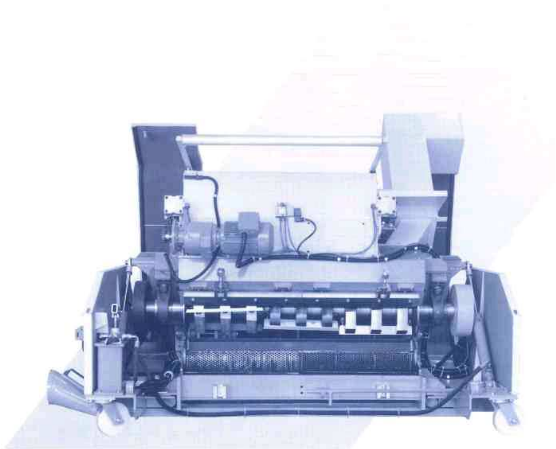
Granulator SML 16/91
