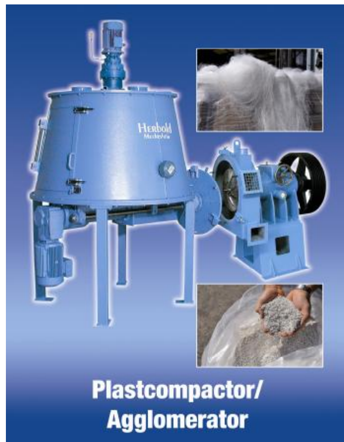
Fig. 5: Plastcompactor Type HV 50
